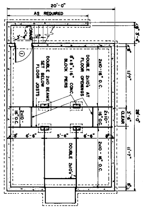
FOUNDATION PLAN
